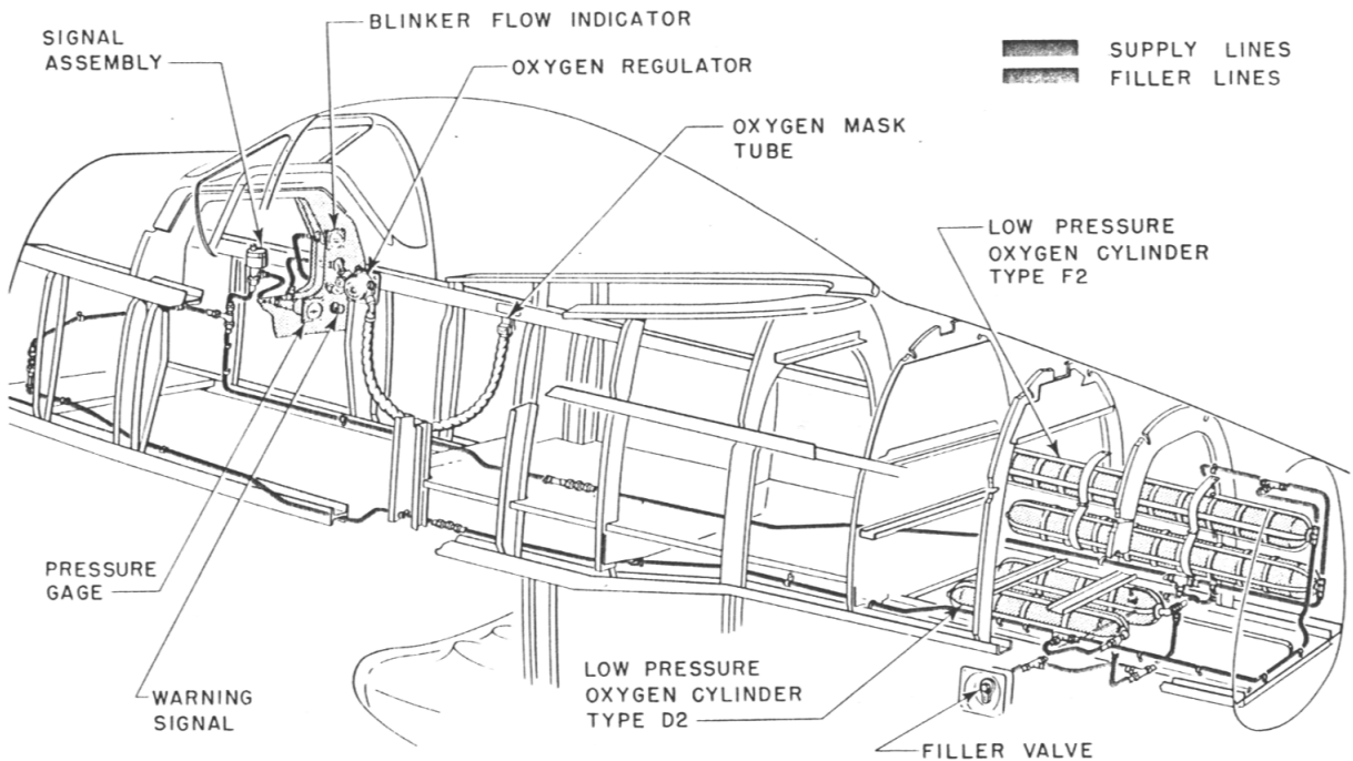
Figure 39—Oxygen System
