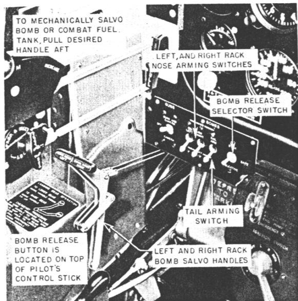
Figure 34—Bomb Controls—Late Airplanes
